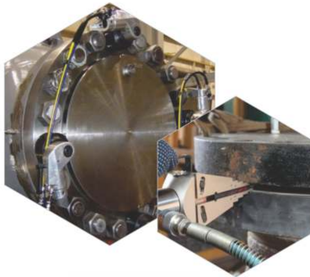
HEX TYPE HYDRAULIC TORQUE WRENCH
